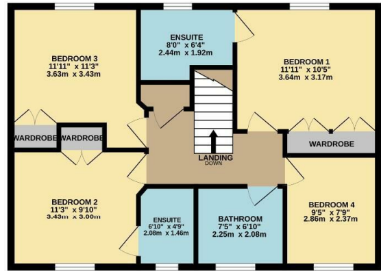
1ST FLOOR 664 sq.ft. (61.7 sq.m.) approx.
